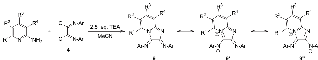
Scheme 4. Synthesis of 4 H -imidazo-[1,2- a ]-pyridines 9 .
