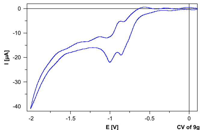
Figure 2. Electrochemical data of different diazapolymethine-merocyanine chromophores and cyclic voltammogram of 9g .
