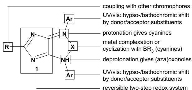
Scheme 1. 4 H -Imidazoles—cyclic merocyanines and functional dyes.
