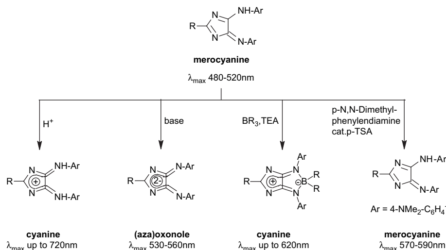
Scheme 3. Derivatization reactions of 4 H -imidazoles.
