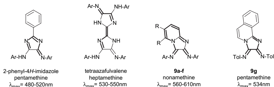
Scheme 5. Diazapolymethine-merocyanines based on cycloamidines.
