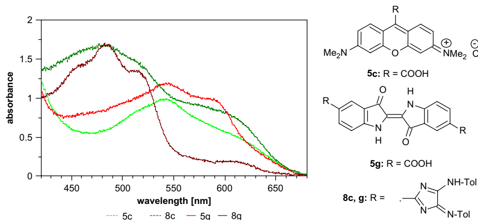
Figure 1. UV-vis spectra of integrated chromophores 5c, g and obtained bichromophores 8c, g .
